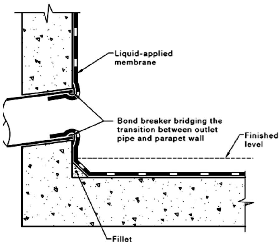
(a) Overflow through parapet
