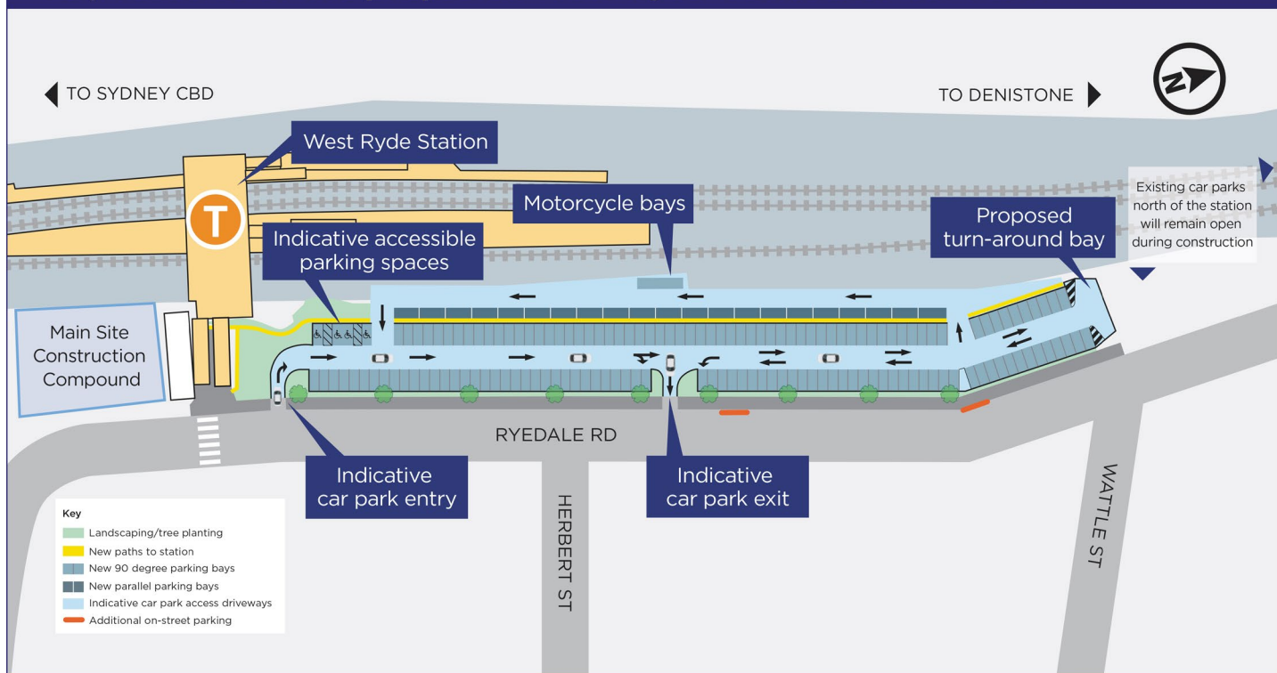
Site map of the new commuter car park, subject to detailed design
