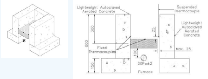
Figure 5.16: Test set up 'A' - Block to non-combustible material
