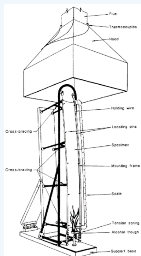
Figure 5.12: Flammability Apparatus (AS 1530.2)
