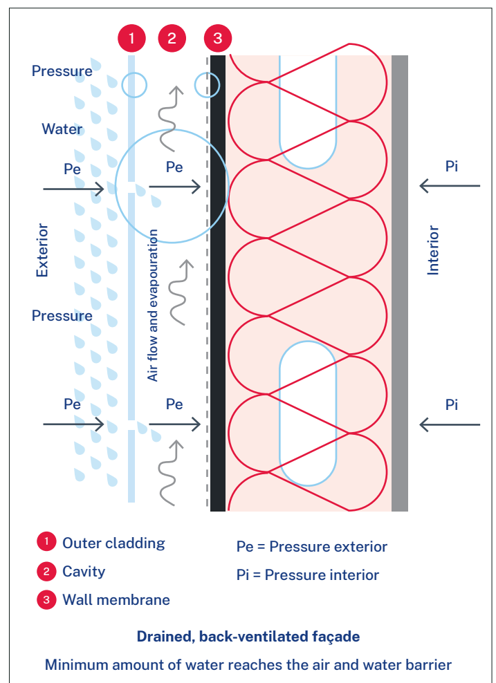
Figure 16.1: The key features of a rain screen
