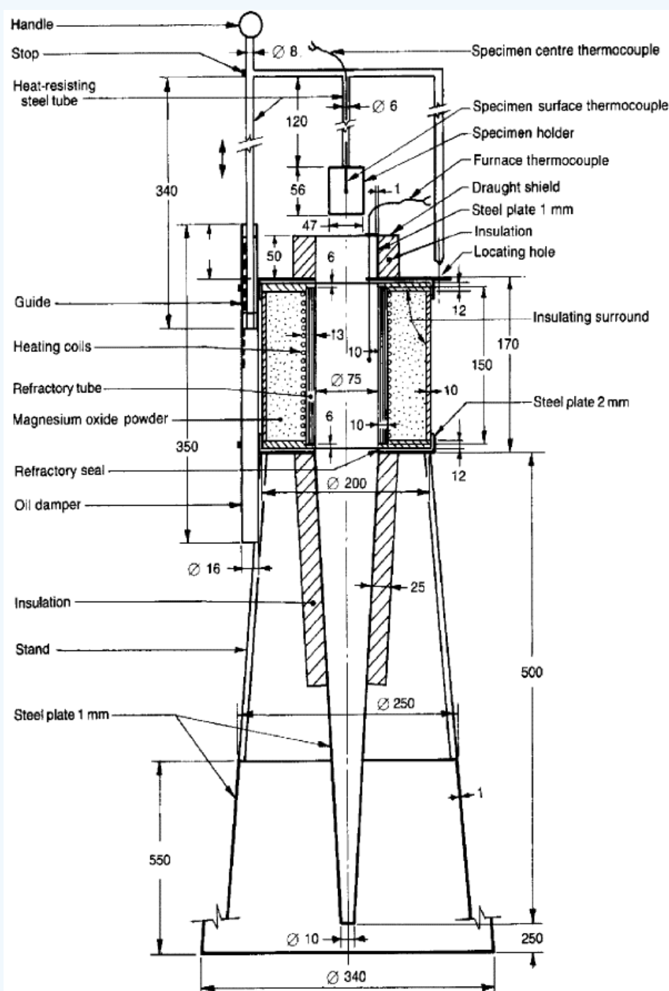
Figure 5.10: Combustibility Apparatus (AS 1530.1)
