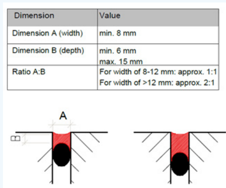
Figure 16.1: Examples of typical joint proportions
