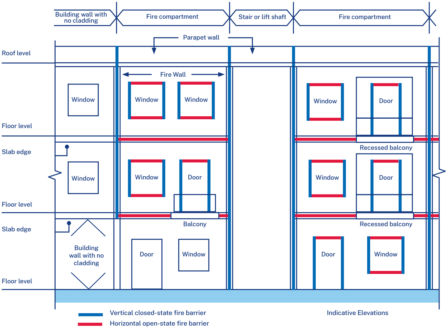
Figure 10.4: Locations of cavity barriers
