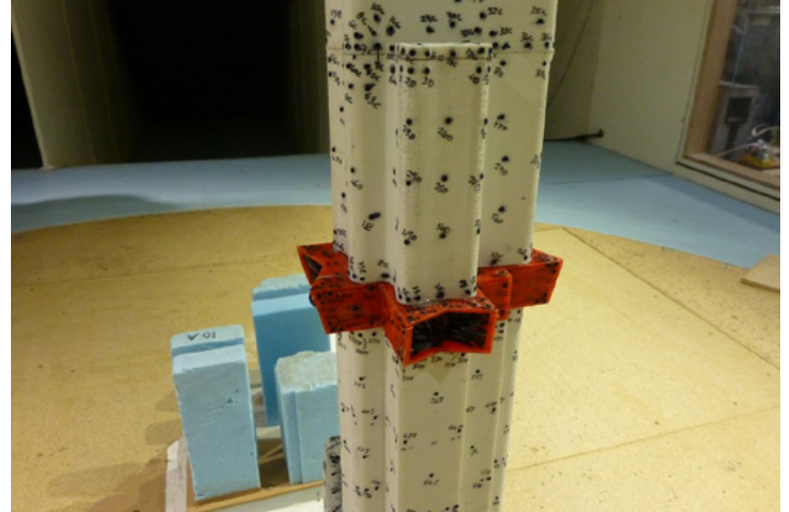
Figure 14.5: Wind Tunnel Testing - Pressure taps at architectural feature locations
