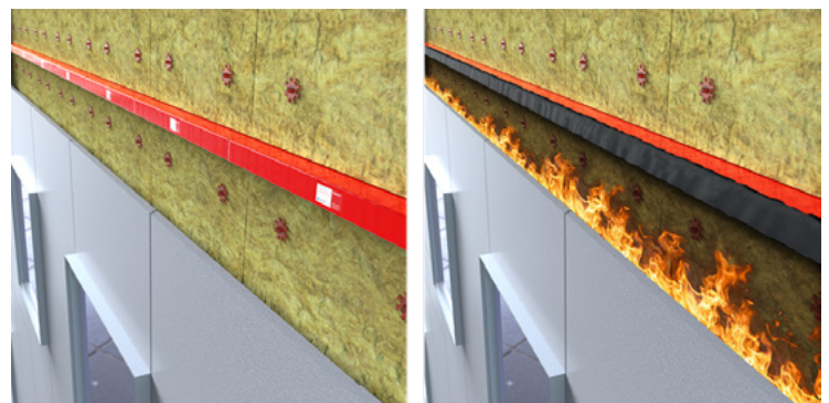
Figure 10.1: Open-state cavity barrier before and after activation
