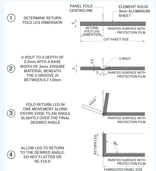
Figure 16.5: Folding of aluminium sheet using routing techniques
