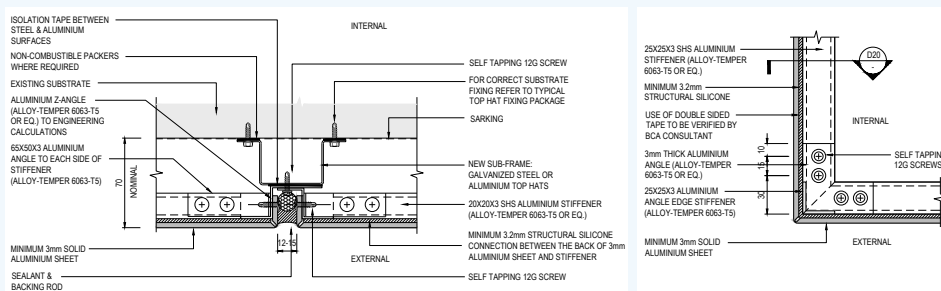
Figure 16.6: Example: V-groove return strengthening method (Pattern Book)
