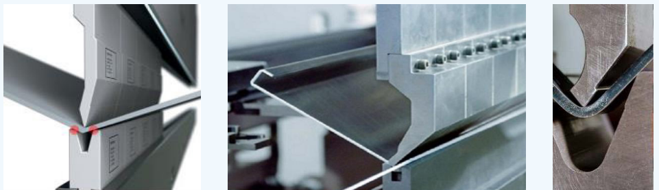
Figure 16.4: Folding of aluminium sheet using mechanical methods including break pressing
