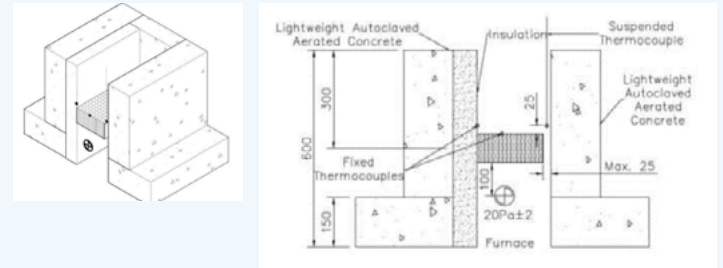
Figure 5.19: Test set up 'D' - Block with uninterrupted insulation to non-combustible material
