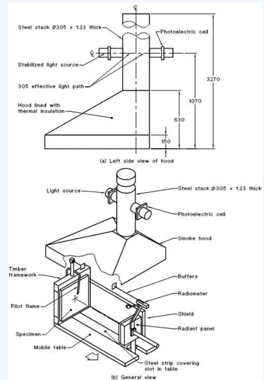
Figure 5.13: Ignitability, Flame Propagation, Heat and Smoke Release Testing Apparatus (AS 1530.3) – Left and General View
