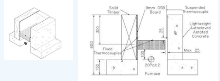
Figure 5.17: Test set up 'B' - Timber frame to non-combustible material
