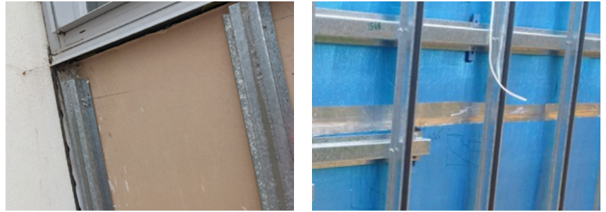
Figure 15.7: Inadequate fire protection and detailing
