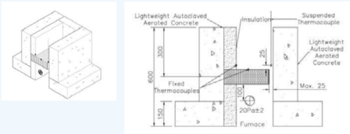
Figure 5.18: Test set up 'C' - Block with interrupted insulation to non-combustible material
